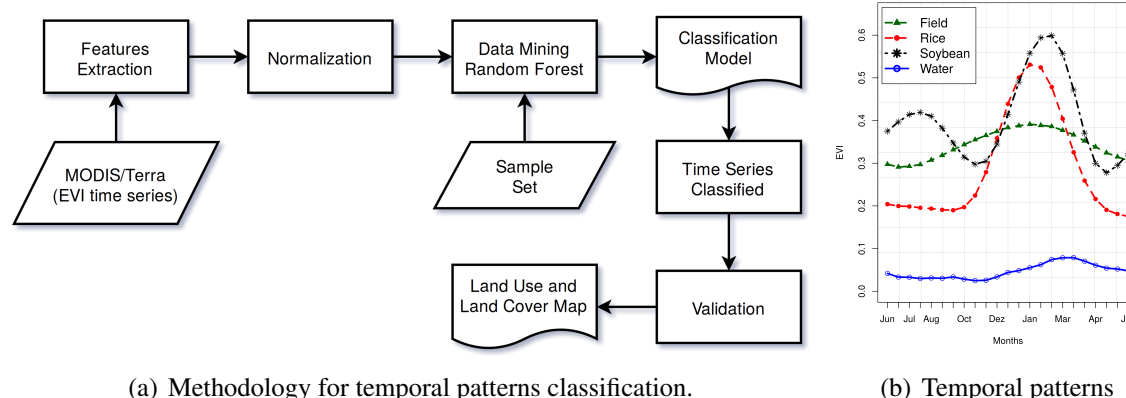
Figure 2: Classification experiment.
