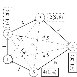
Fig. 1 Left: a TTP instance having 5 cities (circles) and 4 items (rectangles) and a TTP solution with the travelled cyclic path (solid lines) and collected items (solid rectangles). Each city has a city index. City 1 (double circle) is the designated city to start from and end to. Each item has an item index and a tuple for weight and profit. Lines have distances as labels. Dashed lines are not in the travelled path and dotted rectangles are for items not collected. Right: other required parameters of the TTP instances along with the calculation of the net profit for the TTP solution
