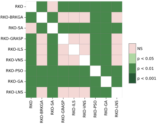
Heat map of the results (p-values) of the Nemenyi test for the RKO methods to solve the NCGPP.
