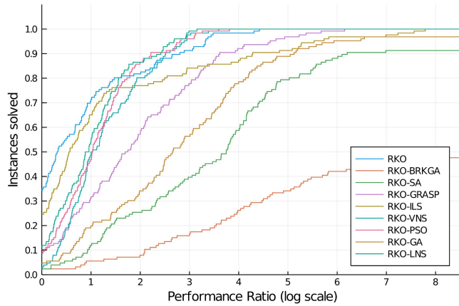
Performance profile of runtime for RKO methods to solve the THLP.
