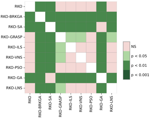
Heat map of the results (p-values) of the Nemenyi test for the RKO methods to solve the THLP.
