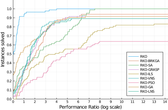
Performance profile of runtime for RKO methods to solve the NCGPP.
