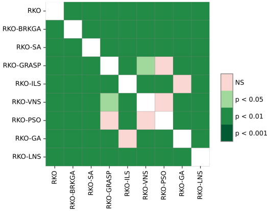
Heat map of the results (p-values) of the Nemenyi test for the RKO methods to solve the \alpha NpMP.
