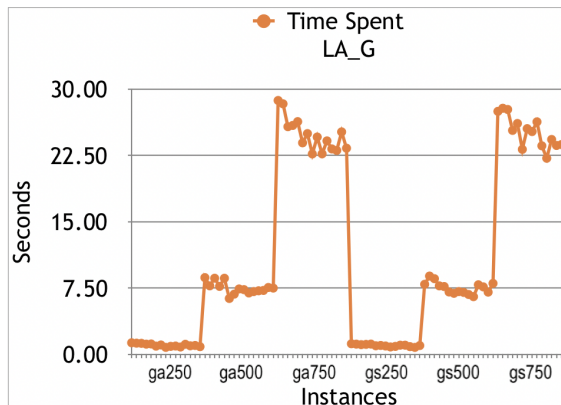
Figure 4: Time to build the initial solution with the Greedy and to run the LA algorithm.
