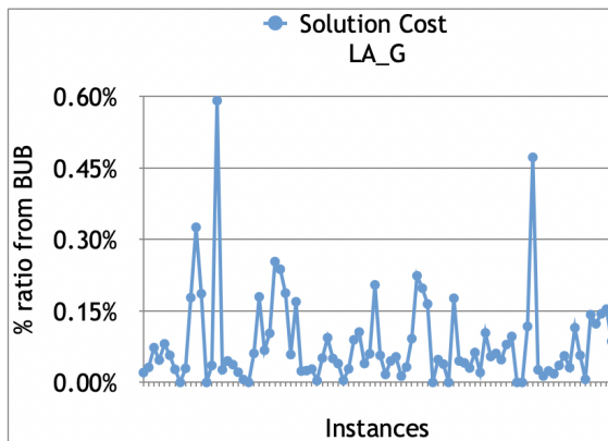
Figure 3: Comparison of the costs achieved by the LA algorithm with the BUB.
