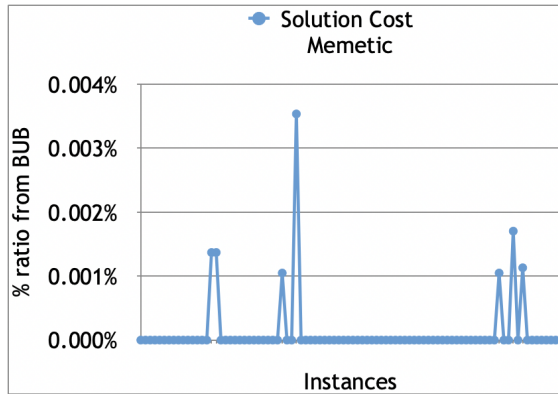
Figure 5: Comparison of the costs achieved by the MA with the BUB.
