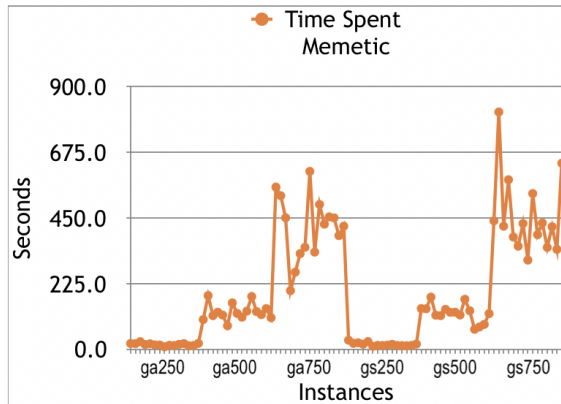
Figure 6: The time to run the Memetic Algorithm.
