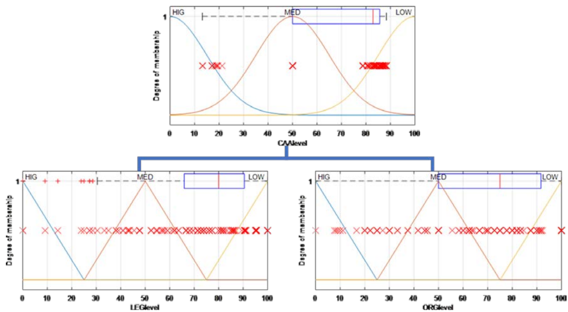
Figure 8 – Membership functions for CAA Branch
