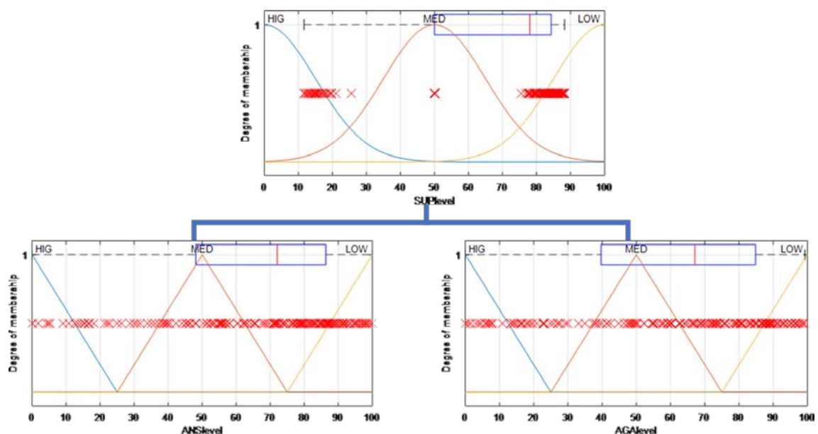
Figure 9 – membership functions for SUP Branch
