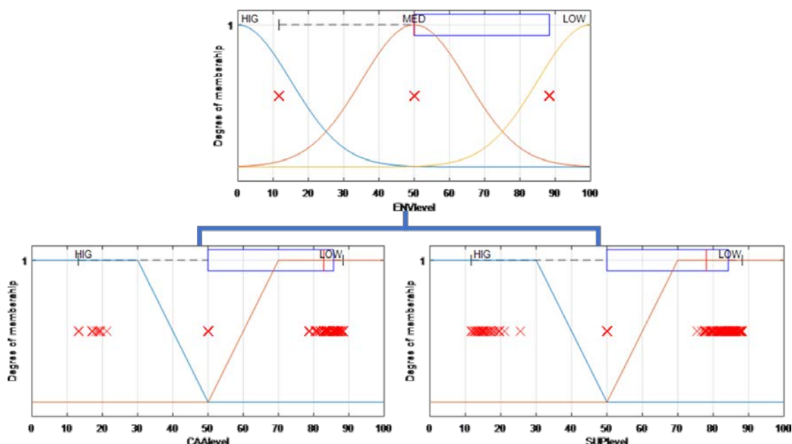
Figure 10 - membership functions for ENV super Branch
