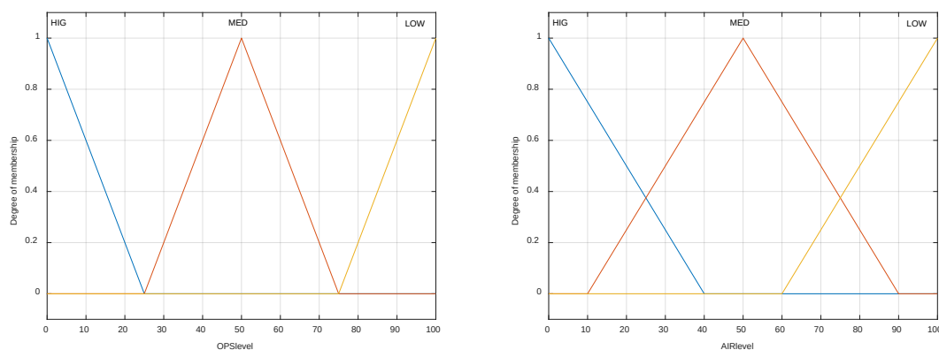
Figure 6 – One set of MF with no intersection (OPSlevel), one set with intersection (AIRlevel)
